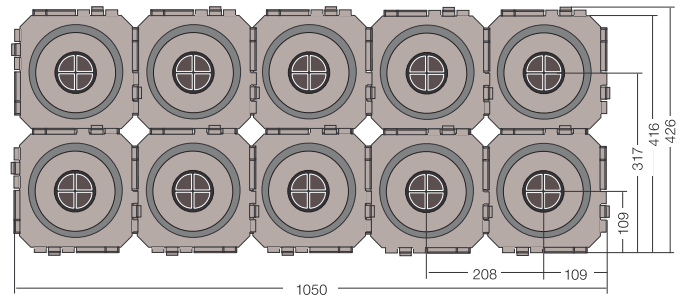
BKD 150-2x5-K2/(L)
