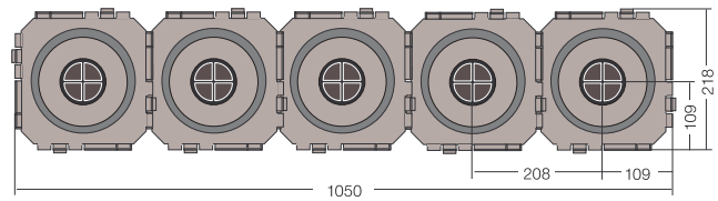
BKD 150-2x5-K2/(L)
